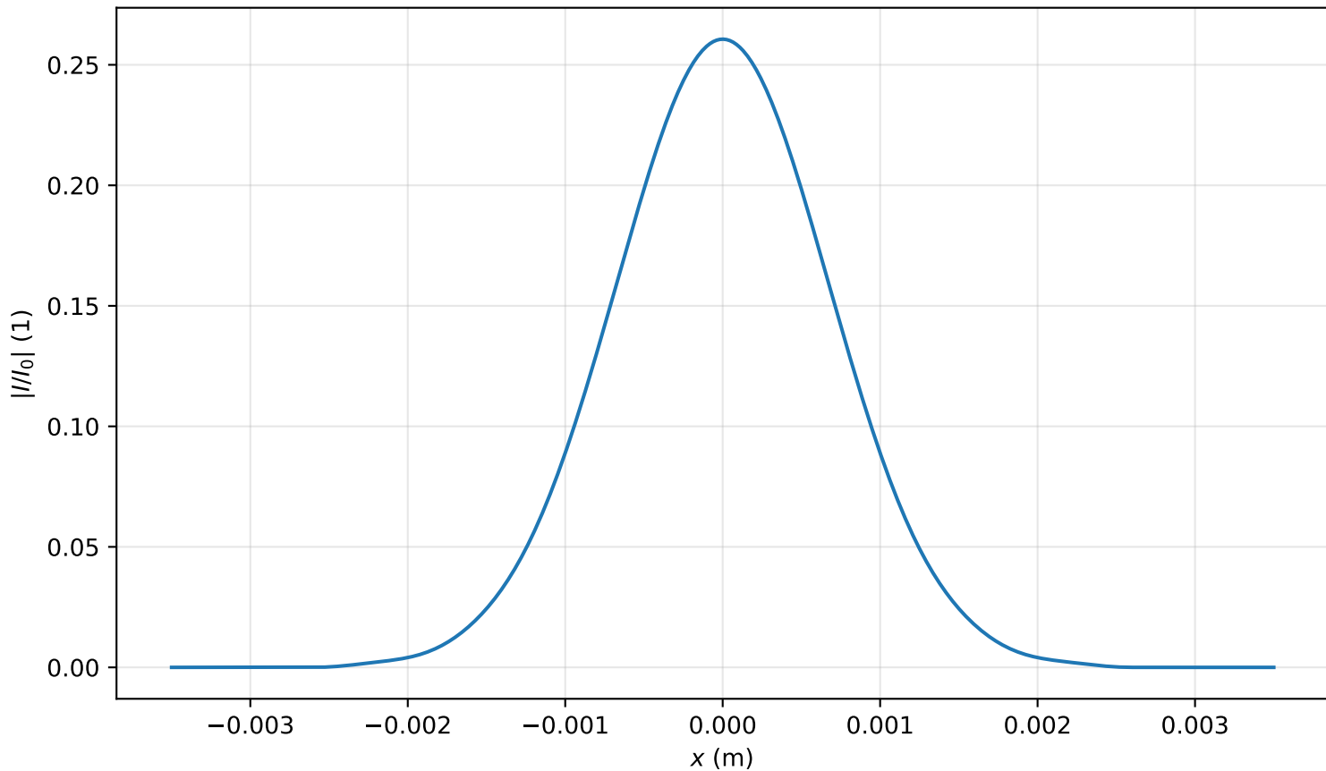
Intensity profile I(x, y = 0, z = 3.582m)/I_0 , P_{in}=0.1P_{cr} , artificial time
